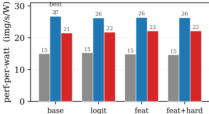
Legion RTX 5070 Ti (GPU-package power)
