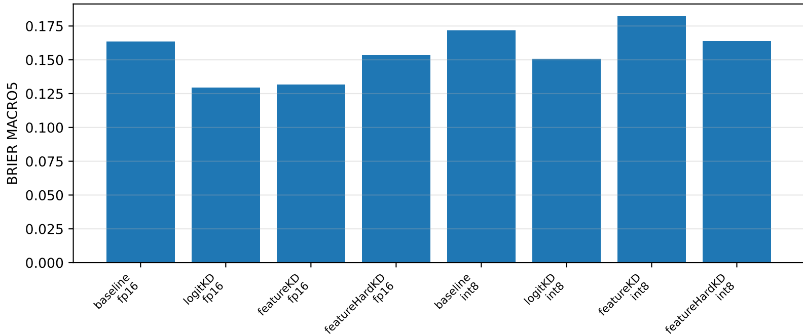
BRIER MACRO5 — jetson, competition classes
