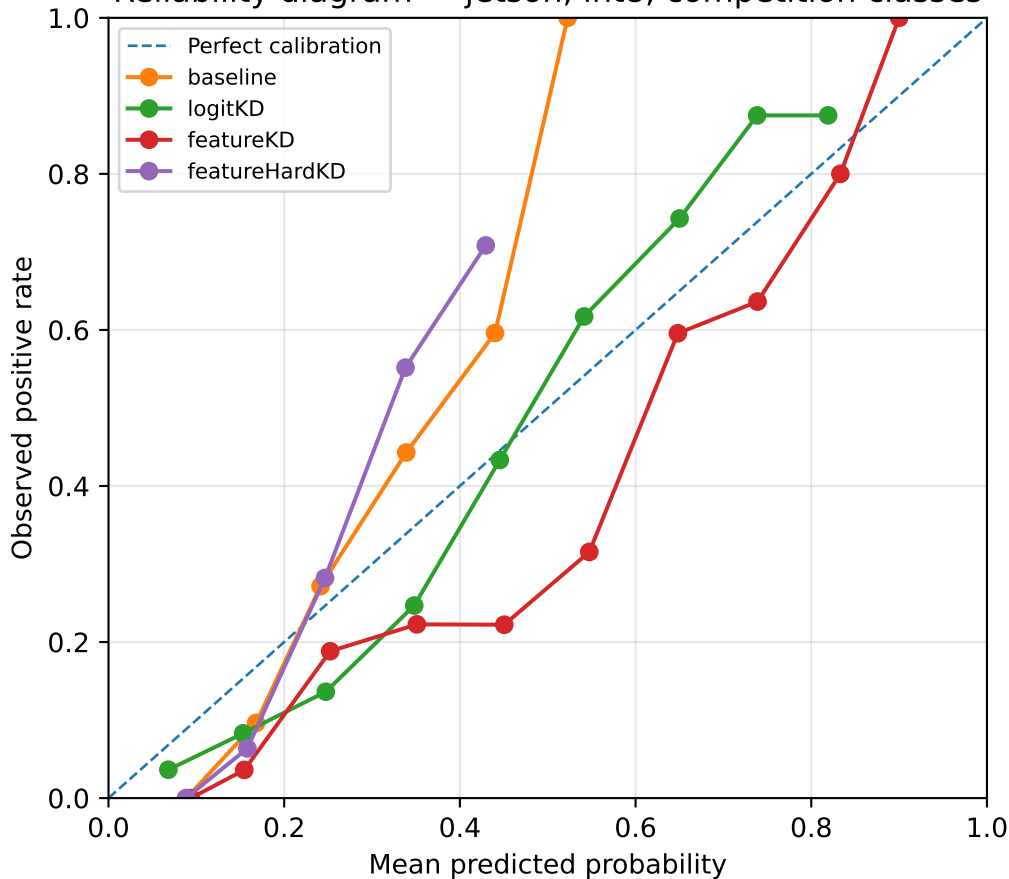
Reliability diagram — jetson, int8, competition classes
