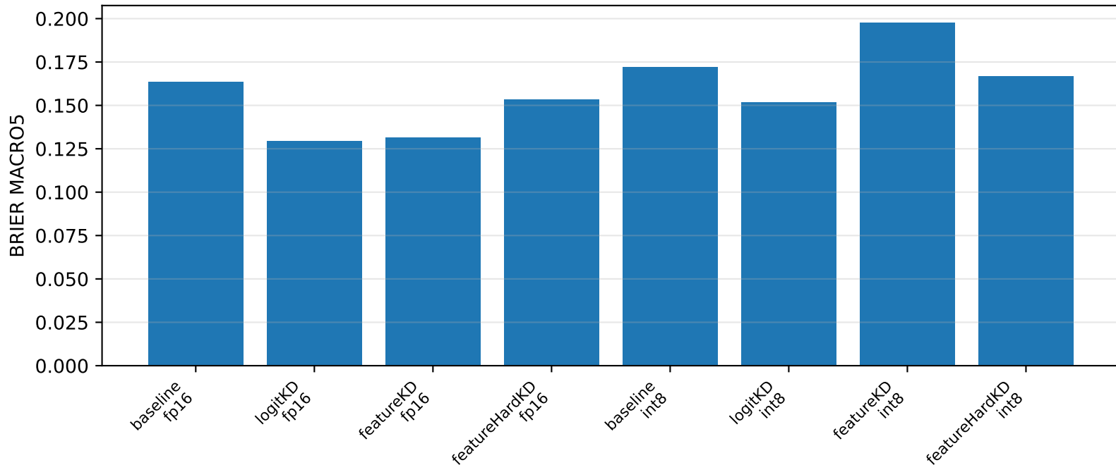
BRIER MACRO5 — legion, competition classes
