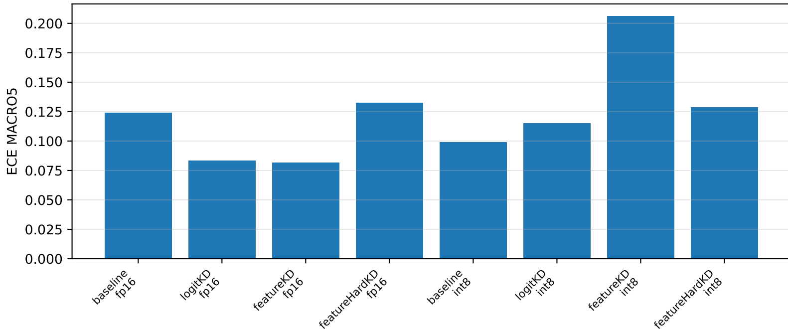
ECE MACRO5 — legion, competition classes
