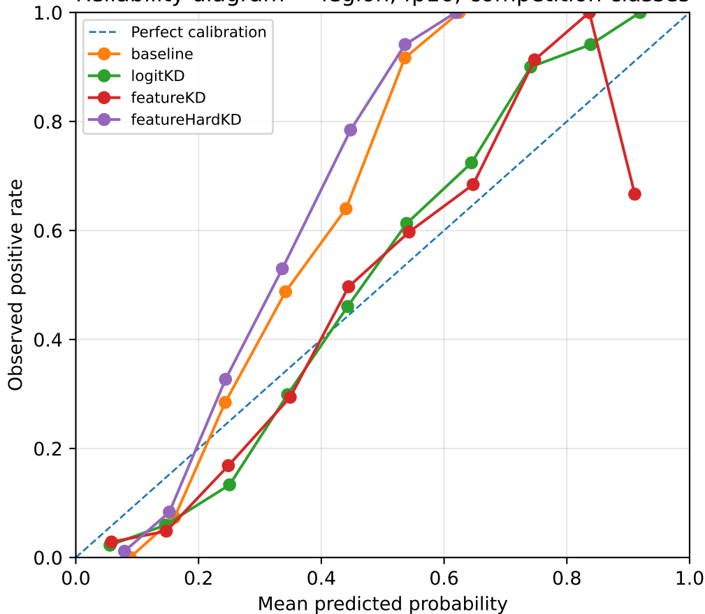
Reliability diagram — legion, fp16, competition classes
