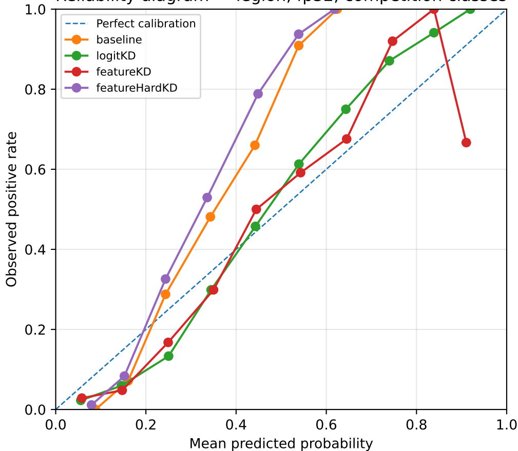
Reliability diagram — legion, fp32, competition classes
