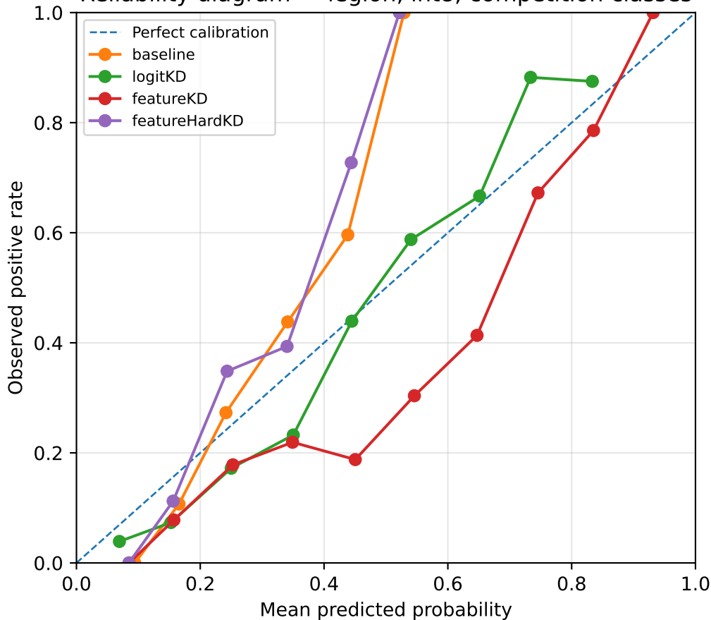
Reliability diagram — legion, int8, competition classes
