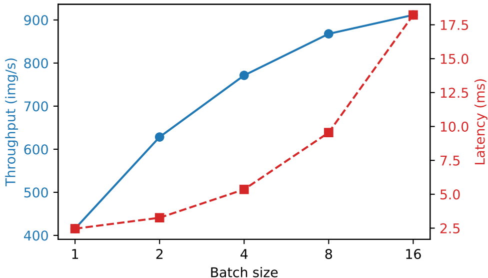
Throughput vs. latency across batch size
