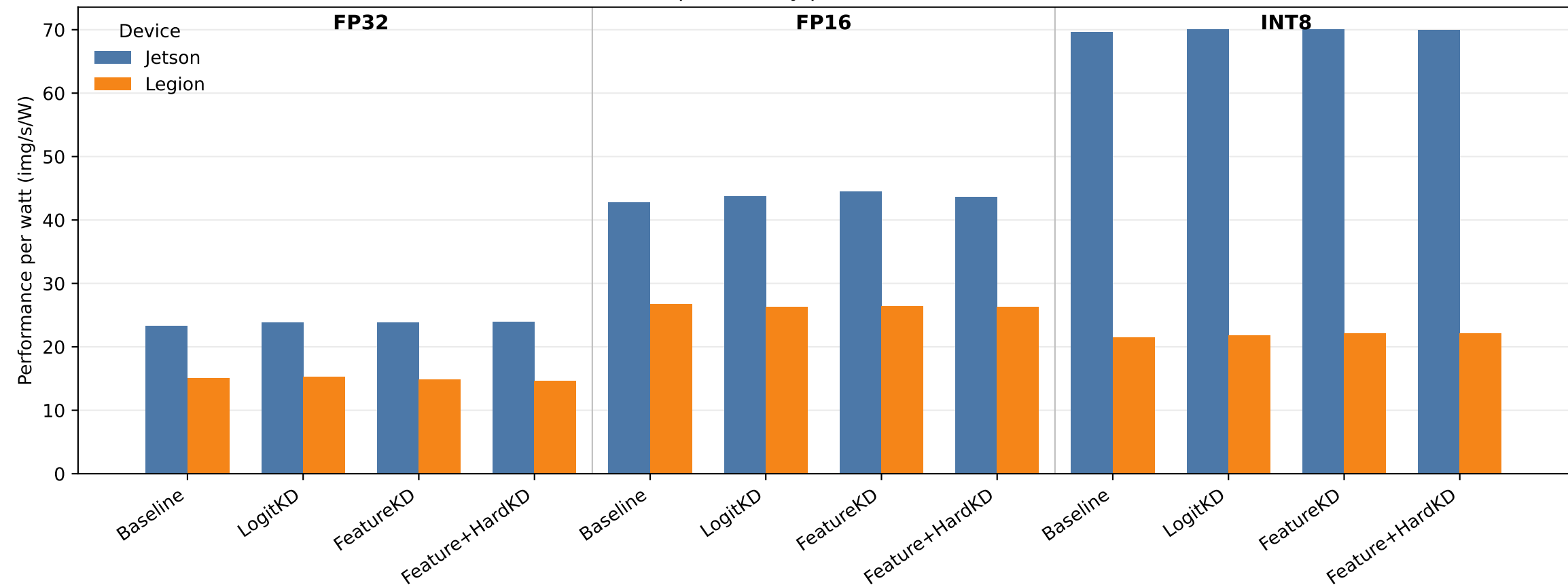
Performance per watt by precision and model variant
