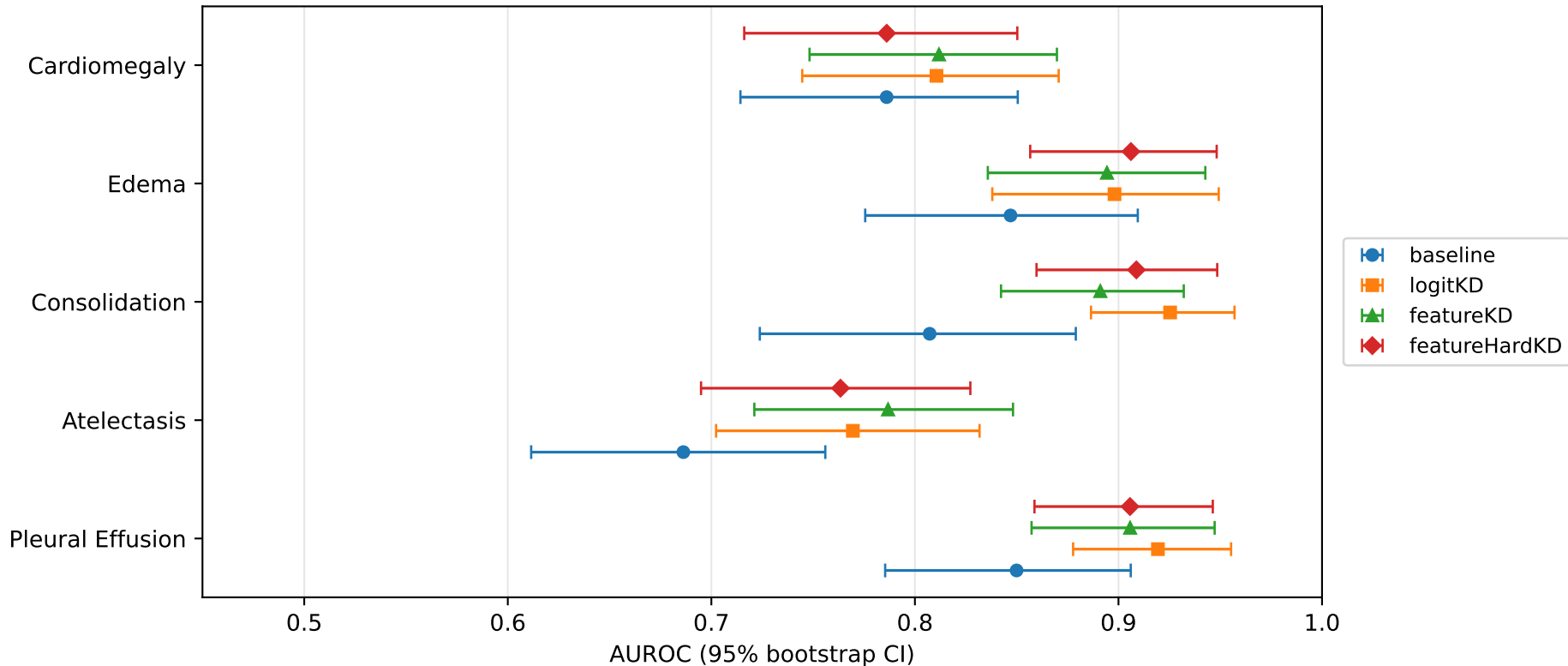
Per-class AUROC - jetson FP16 Image-level AUROC; patient-cluster bootstrap CI
