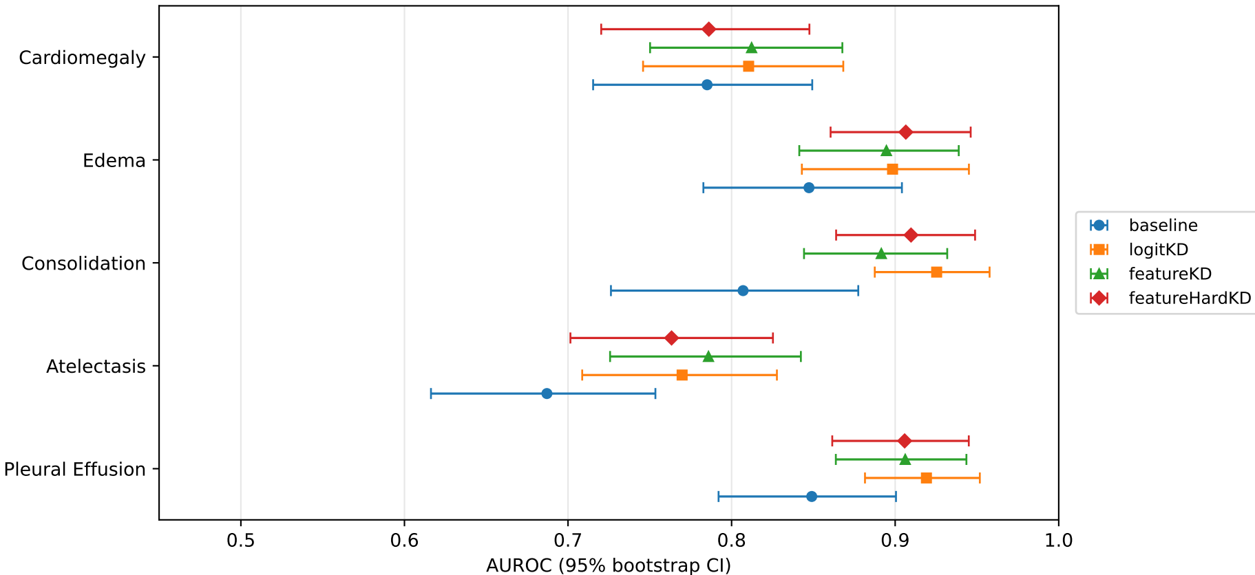
Per-class AUROC - legion FP16 Image-level AUROC; image bootstrap CI
