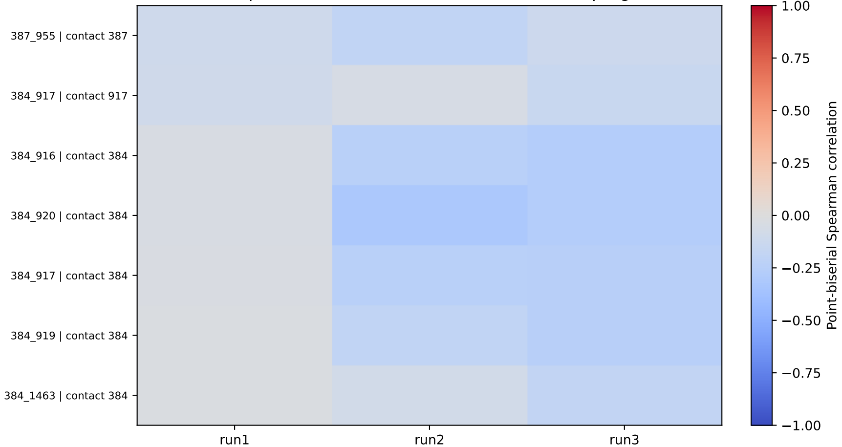
Replica-consistent distance/ProLIF contact coupling
