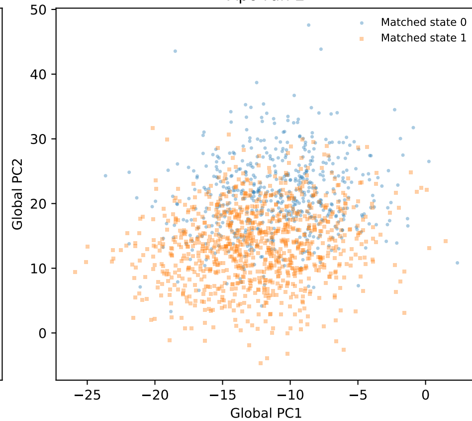
Apo run 2
