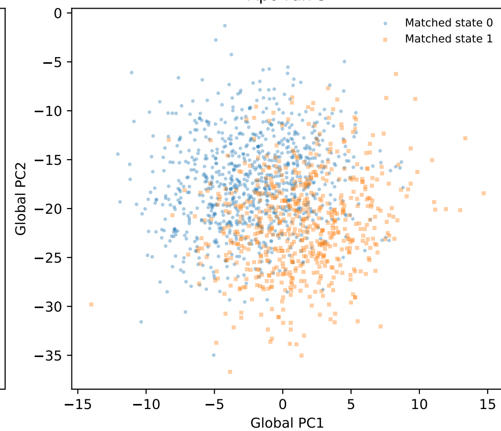
Apo run 3
