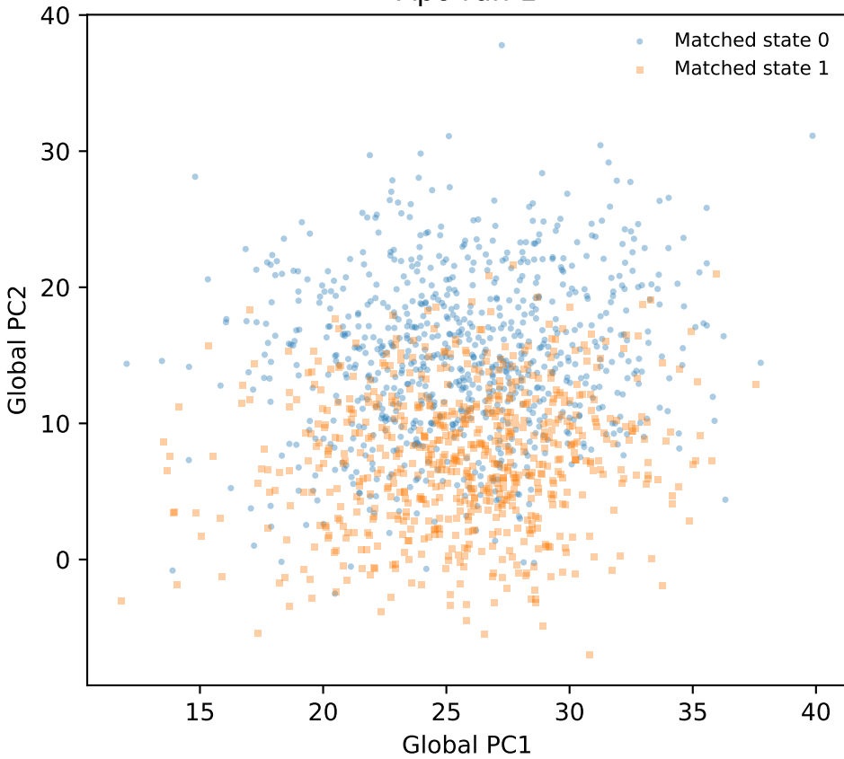
Apo run 1
