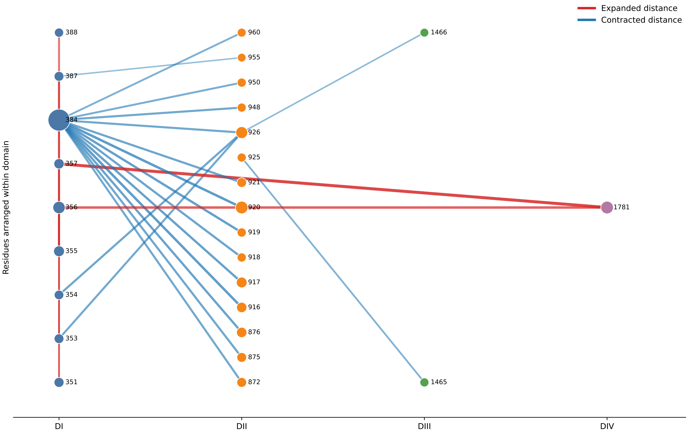
Z944 vs Apo reproducible distance network red = expansion; blue = contraction
