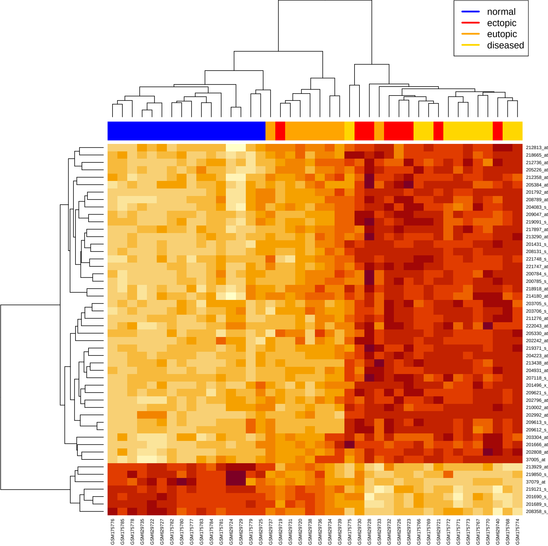
Top 50 DEGs: Ectopic vs. Normal
