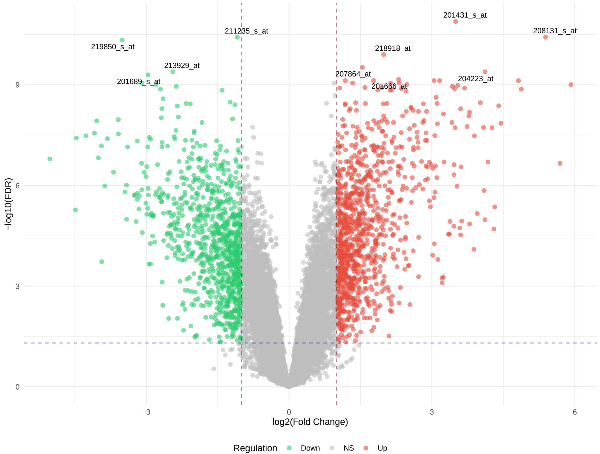
diseased vs normal – Volcano Plot
