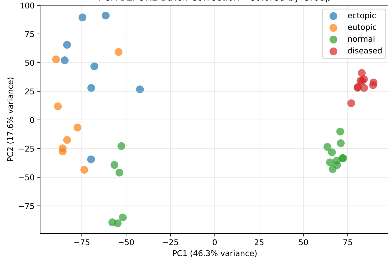
PCA BEFORE Batch Correction - Colored by Group
