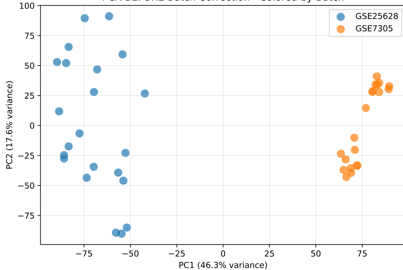
PCA BEFORE Batch Correction - Colored by Batch
