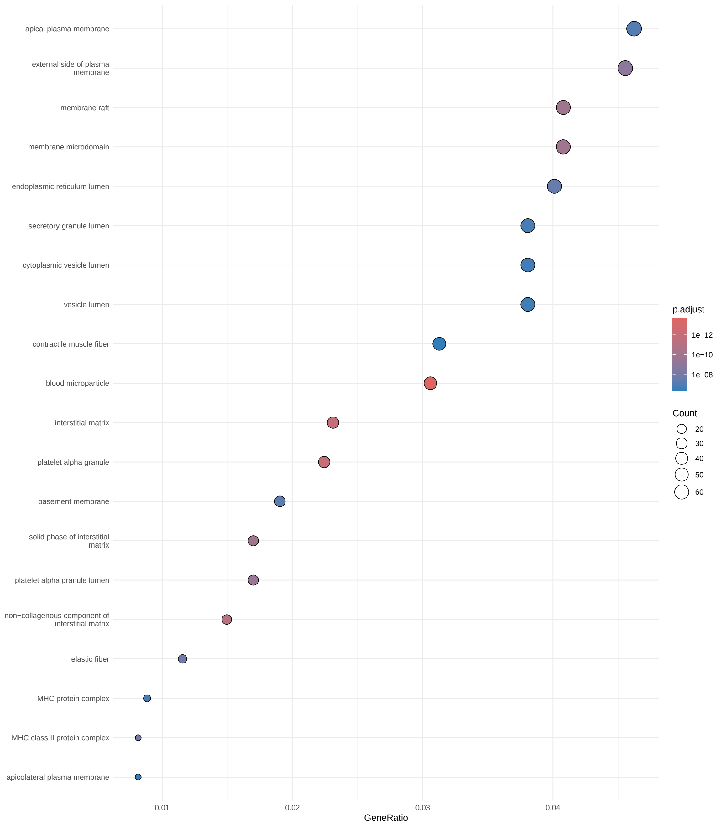
GO Cellular Component: diseased vs normal
