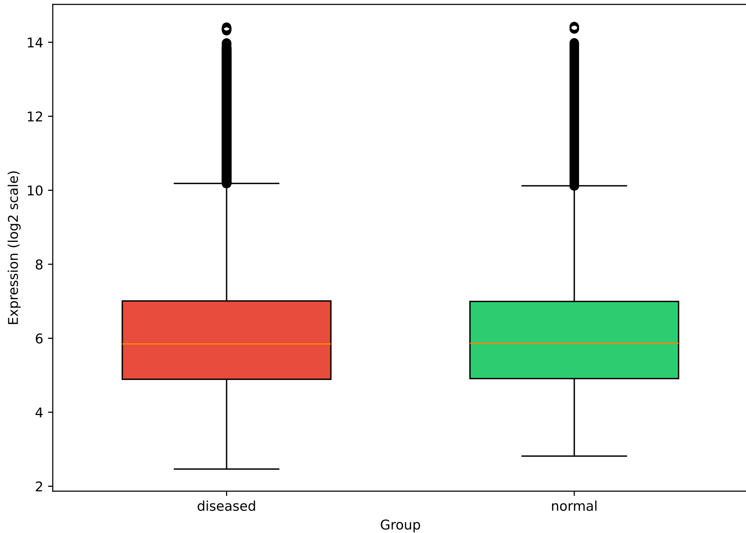
GSE7305: Endometriosis Dataset - Expression by Group
