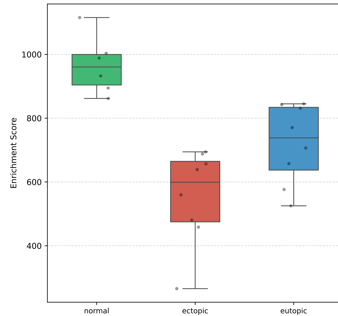
Gse2770 Untreated Vs Il12 Treated Act Cd4 Tcell 48H Up GSE25628 - FDR: 2.48e-02
