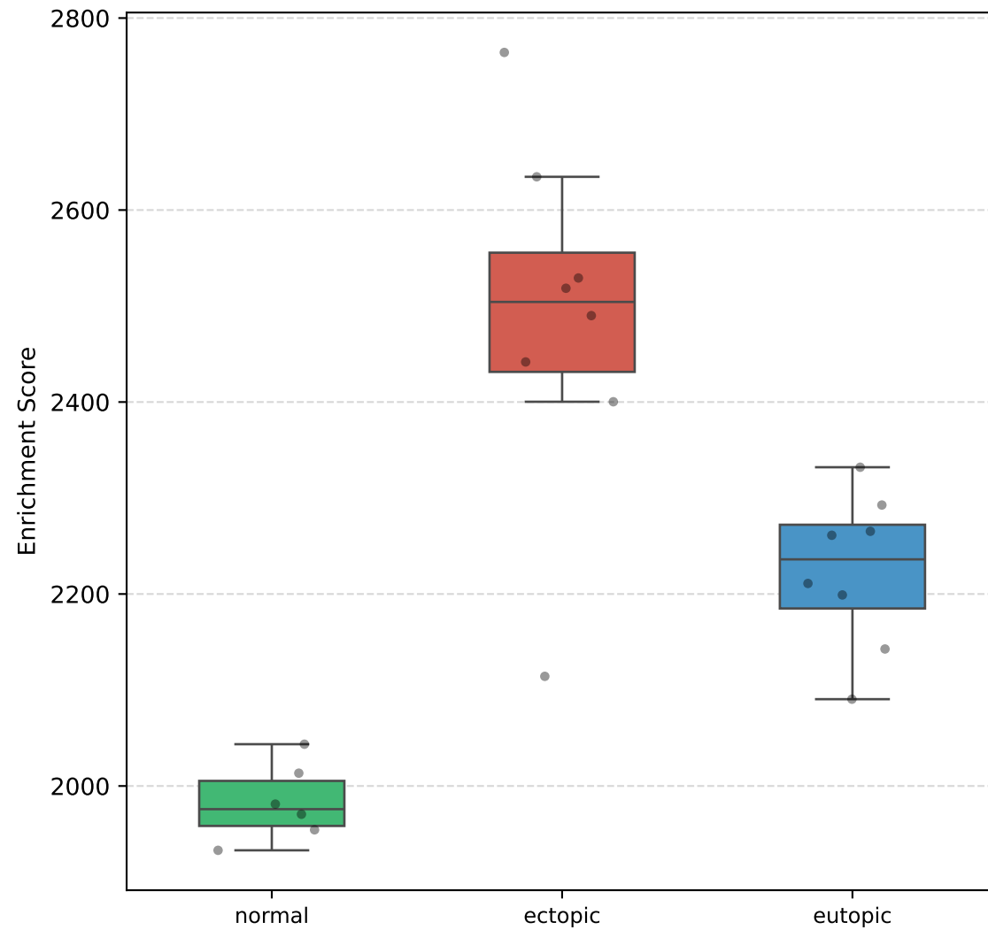
Gse9316 Il6 Ko Vs Ifng Ko Invivo Expanded Cd4 Tcell Up GSE25628 - FDR: 2.48e-02
