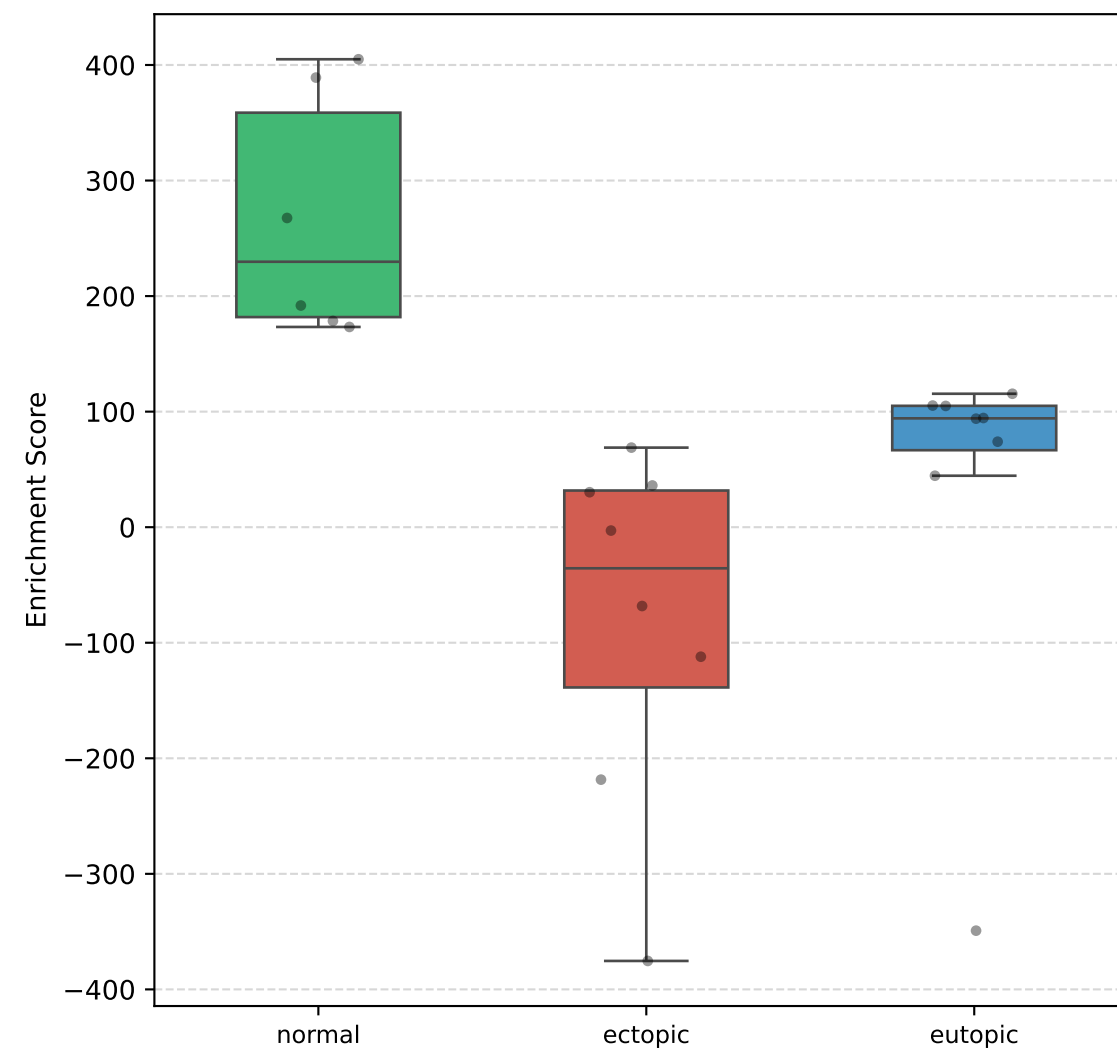
Gse14308 Naive Cd4 Tcell Vs Natural Treg Dn GSE25628 - FDR: 2.48e-02
