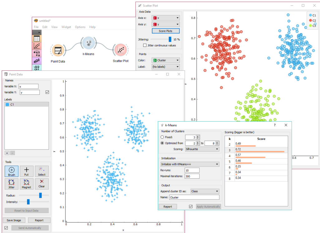
Fig. 2. Example Orange workflow to visualise data, cluster it with K-Means, and then show the clustering [102].
