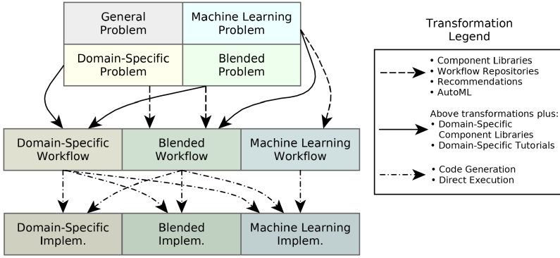
Fig. 10. Transformations among the problem space, solution workflow space, and the implementation space.
