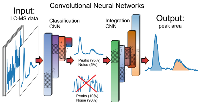
Fig. 11. Visual abstract from Melnikov et al. [90] demonstrating classification and integration of peaks. Figure reprinted (adapted) with permission from Melnikov et al. [90]. Copyright © 2020 American Chemical Society.
