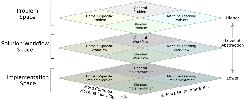
Fig. 4. Our three-layer framework with the problem, solution workflow, and implementation spaces. Each layer is divided into four regions along the DS and complexity of ML dimensions.
