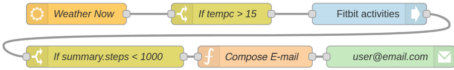
Fig. 1. Example Node-RED flow to send an e-mail when the weather is nice and a step counter is low. The figure is modified from the work of Lea [80].
