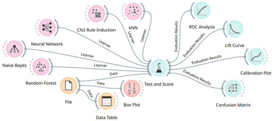
Fig. 12. Solution workflow in the Orange tool. Adapted from the work of Adekitan et al. [1].
