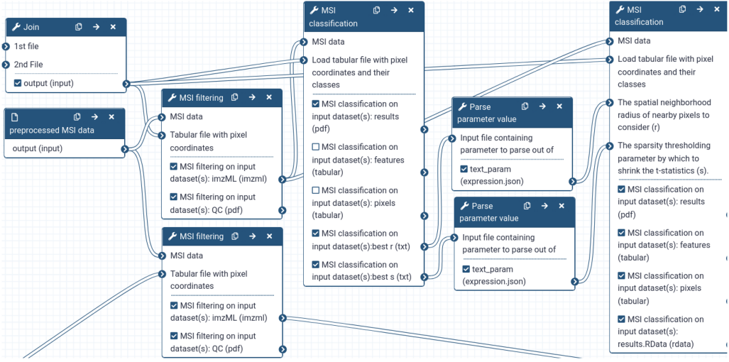
Fig. 3. A selection of a workflow described in the work of Föll et al. [47], in the workflow management tool Galaxy [66].
