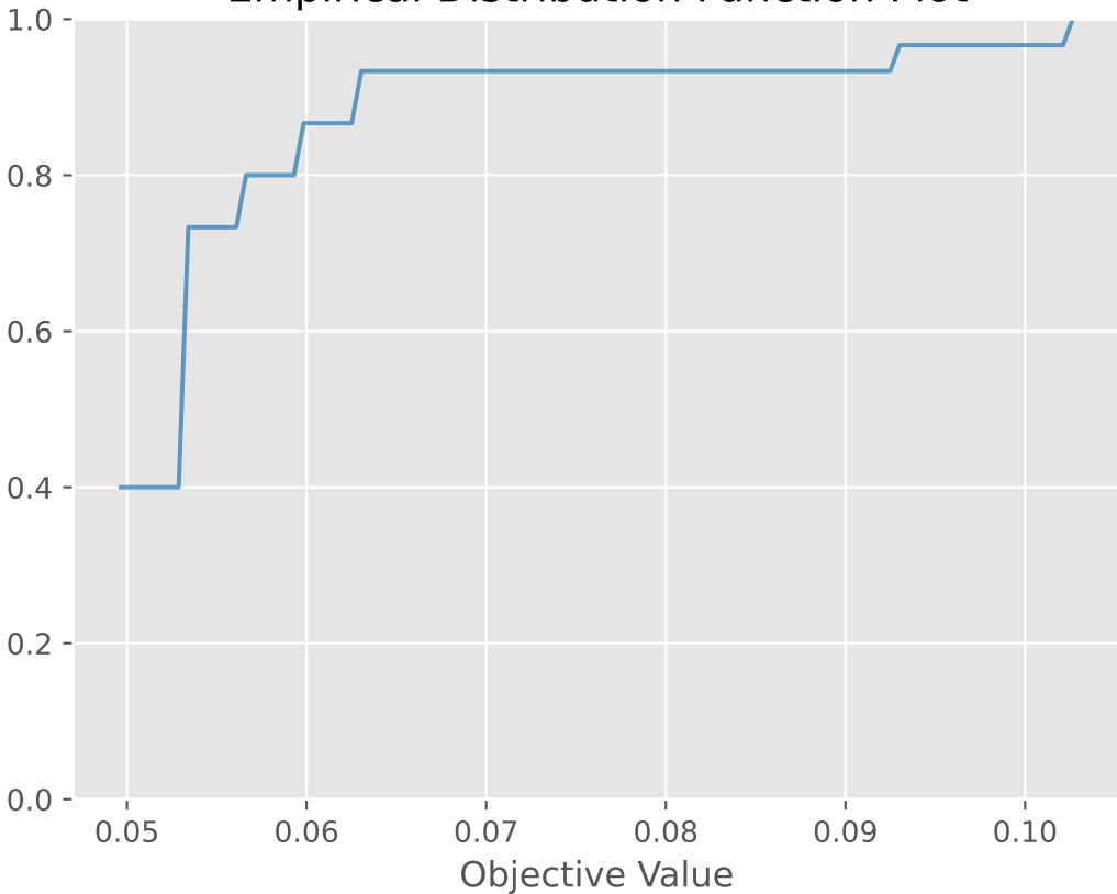
Empirical Distribution Function Plot
