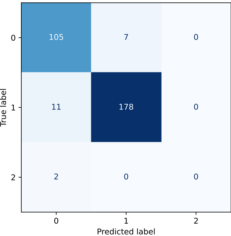
FNN Confusion Matrix
