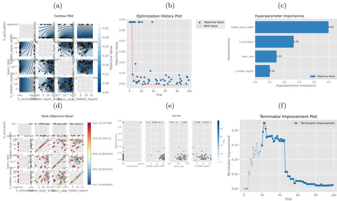
Figure 8: Optuna exploration on FNN hyperparameters. Objective value corresponds to error rate on validation set across all classes.
