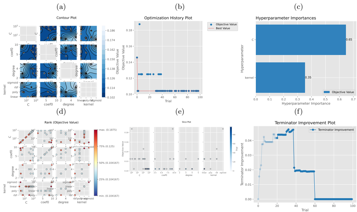
Figure 10: Optuna exploration on SVM hyperparameters. Objective value corresponds to error rate on validation set across all classes.
