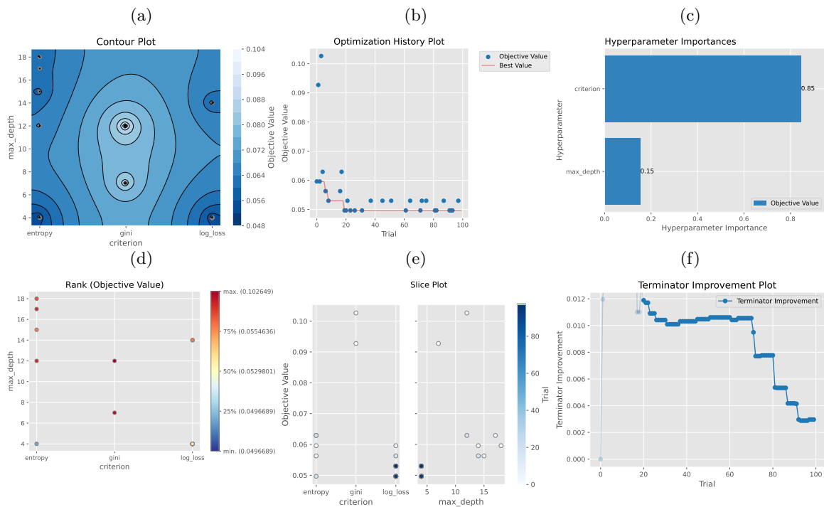
Figure 9: Optuna exploration on DT hyperparameters. Objective value corresponds to error rate on validation set across all classes.
