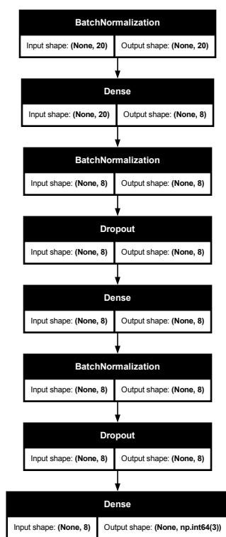
Figure 3: FNN with smallest validation error after 100 trials.
