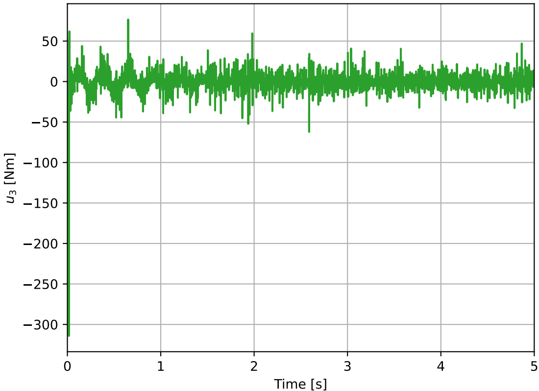
Control torque applied at wrist joint
