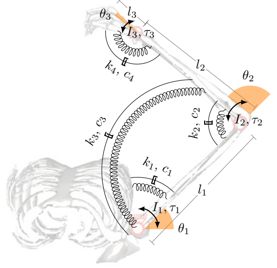
Figure 1. Human upper limb simplified mechanical representation. Adapted from Albuquerque and Machado (2025).
