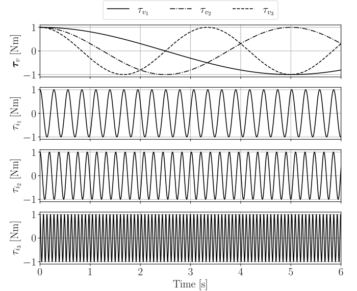
Figure 2. Tremor torque adopted for all simulations and voluntary torque adopted for deliberate motion scenario.
