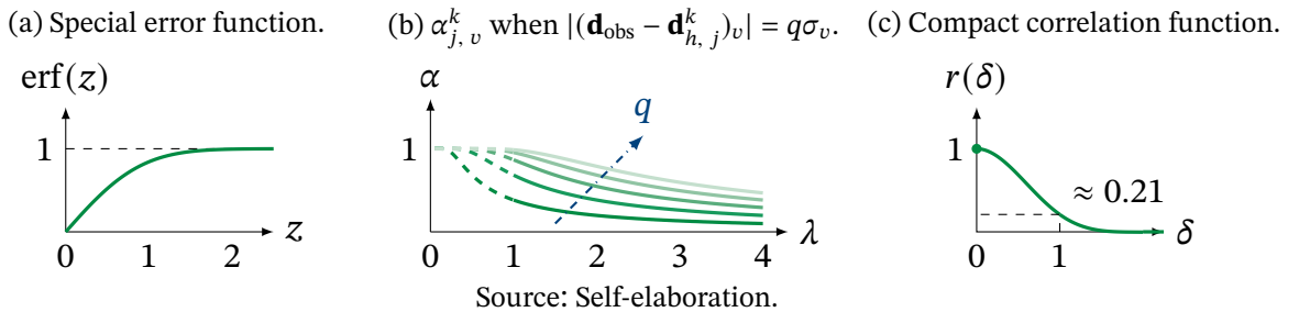
Figure 3.3 – Important functions for understanding the proposed Data-Space Inversion algorithm.
