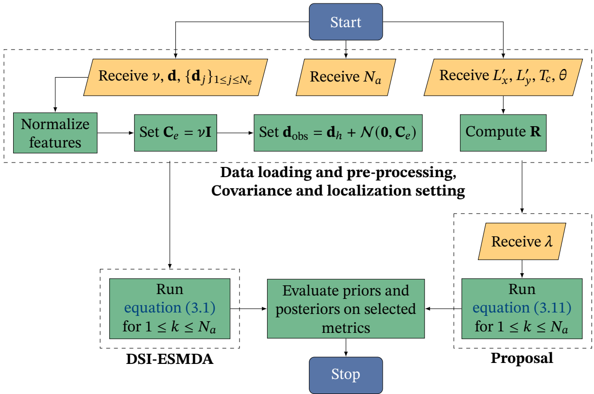
Figure 4.3 – Outline of the evaluation process.
