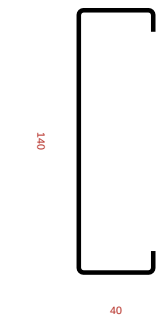
Ue 140x40x12x1,25
