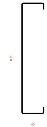
Ue 200x40x12x1,25
