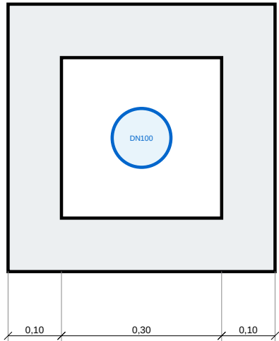
2 SHAFT VERTICAL ESCALA 1:10
