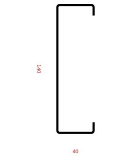
Ue 140x40x12x1,25
