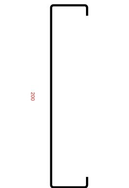
Ue 200x40x12x1,25
