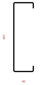
Ue 140x40x12x1,25
