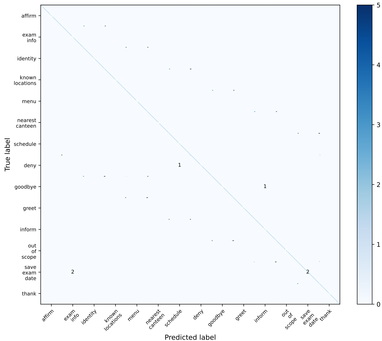
Intent Confusion Matrix (hold-out test set)
