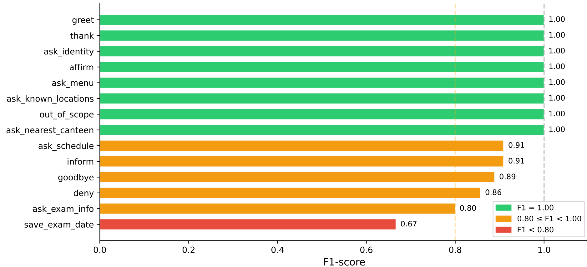
NLU Intent F1-score (hold-out test set, n=63, accuracy=87.3%)
