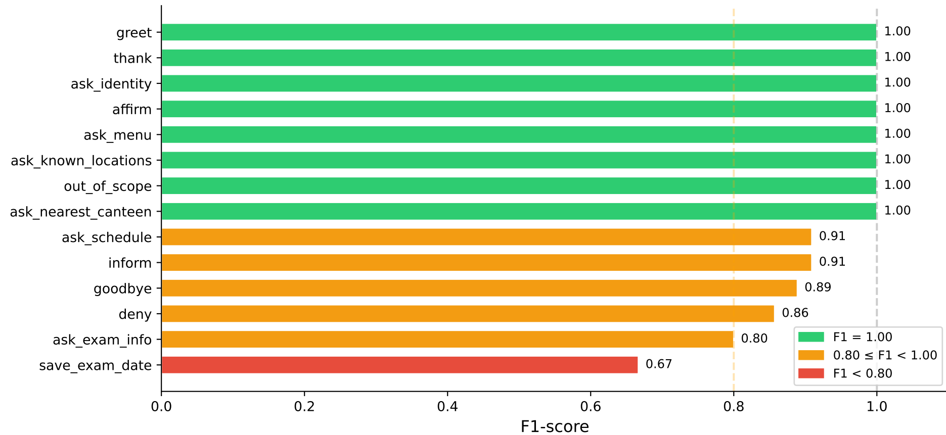
NLU Intent F1-score (hold-out test set, n=63, accuracy=93.7%)
