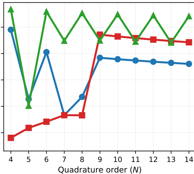
Kumaraswamy (2,2.41)
