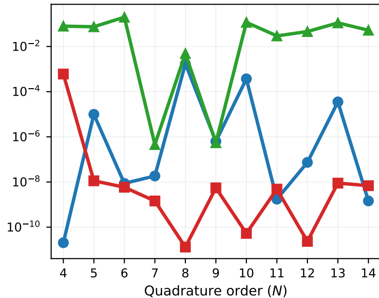
Kumaraswamy (2,8)
