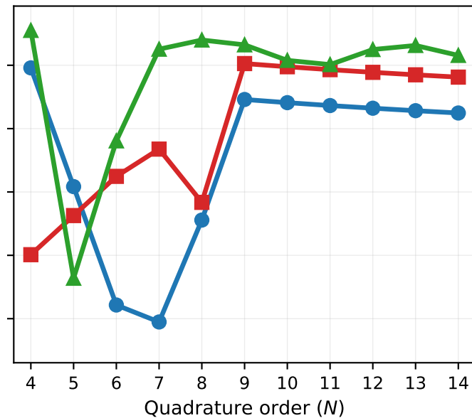
Kumaraswamy (4,1.5)
