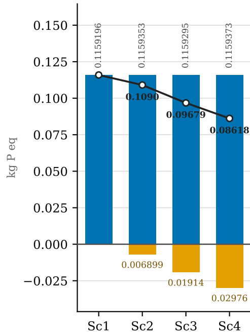
Eutrophication freshwater
