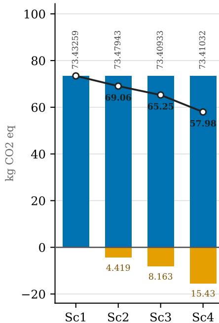
Climate change
