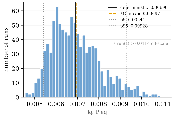
Eutrophication freshwater
