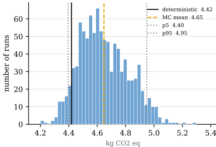
Climate change
