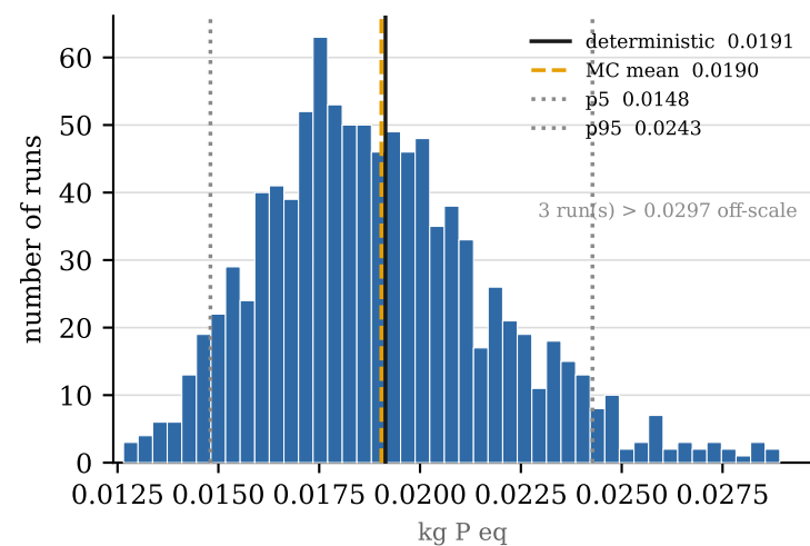
Eutrophication freshwater
