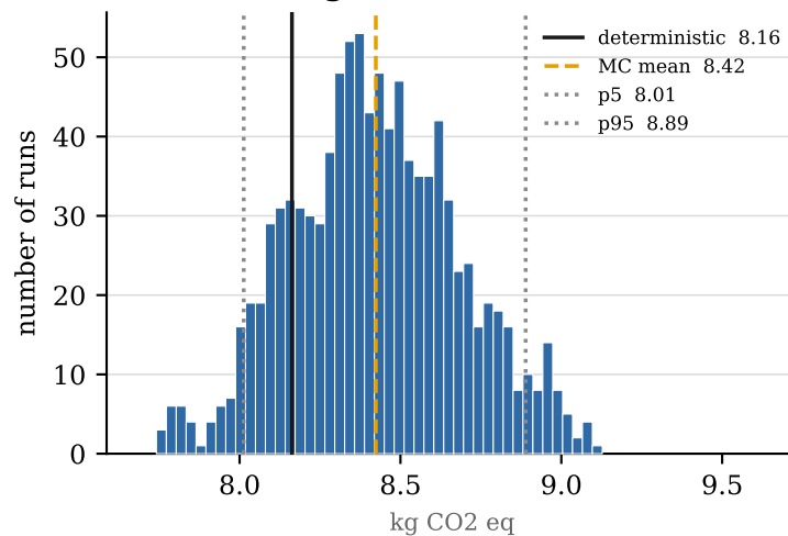
Climate change
