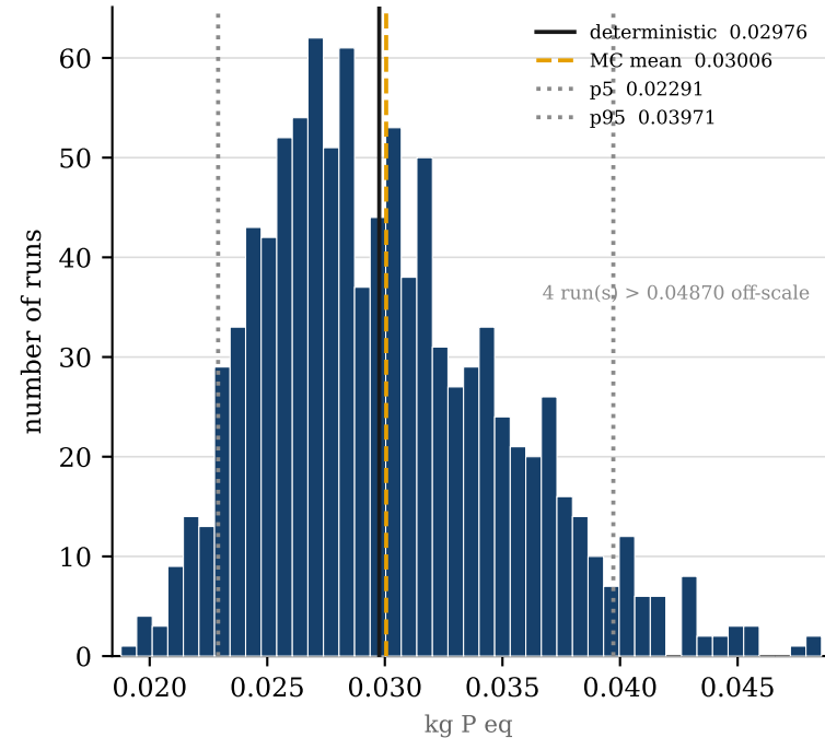
Eutrophication freshwater
