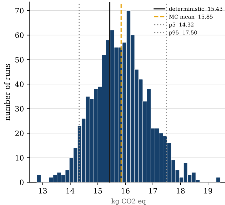
Climate change
