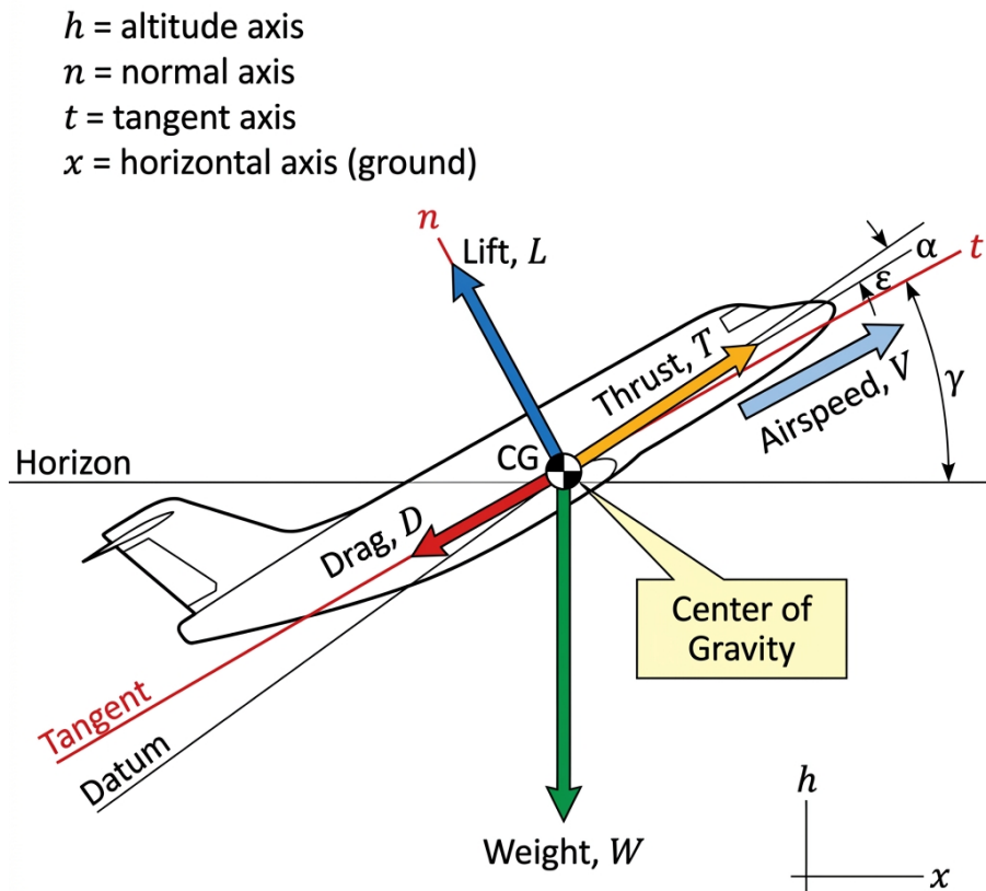
Figure 1: Forces and reference axes acting on an aircraft in climbing flight. The four main forces (Lift L , Drag D , Weight W , Thrust T ) act through the center of gravity, with angles \alpha (angle of attack), \gamma (climb angle), and \epsilon (thrust offset) defined relative to the flight path and horizon.
