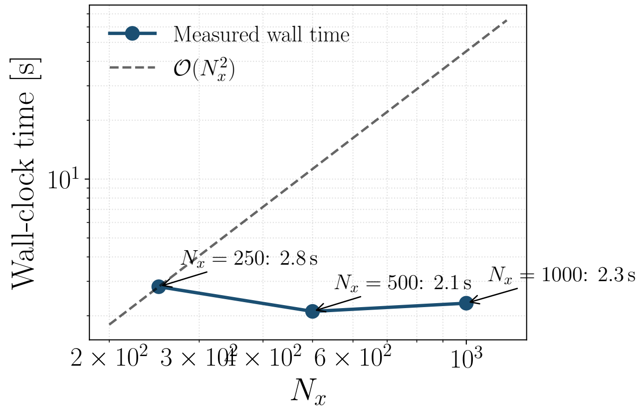
KT solver execution time vs resolution
