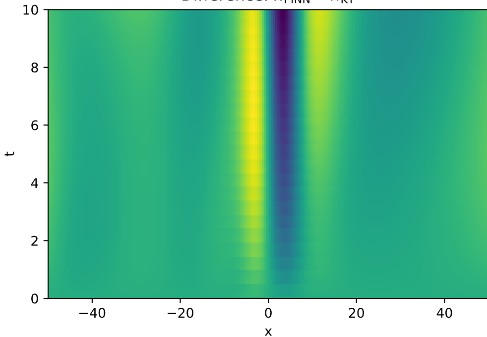
Difference: n_{\text{PINN}} - n_{\text{KT}}
