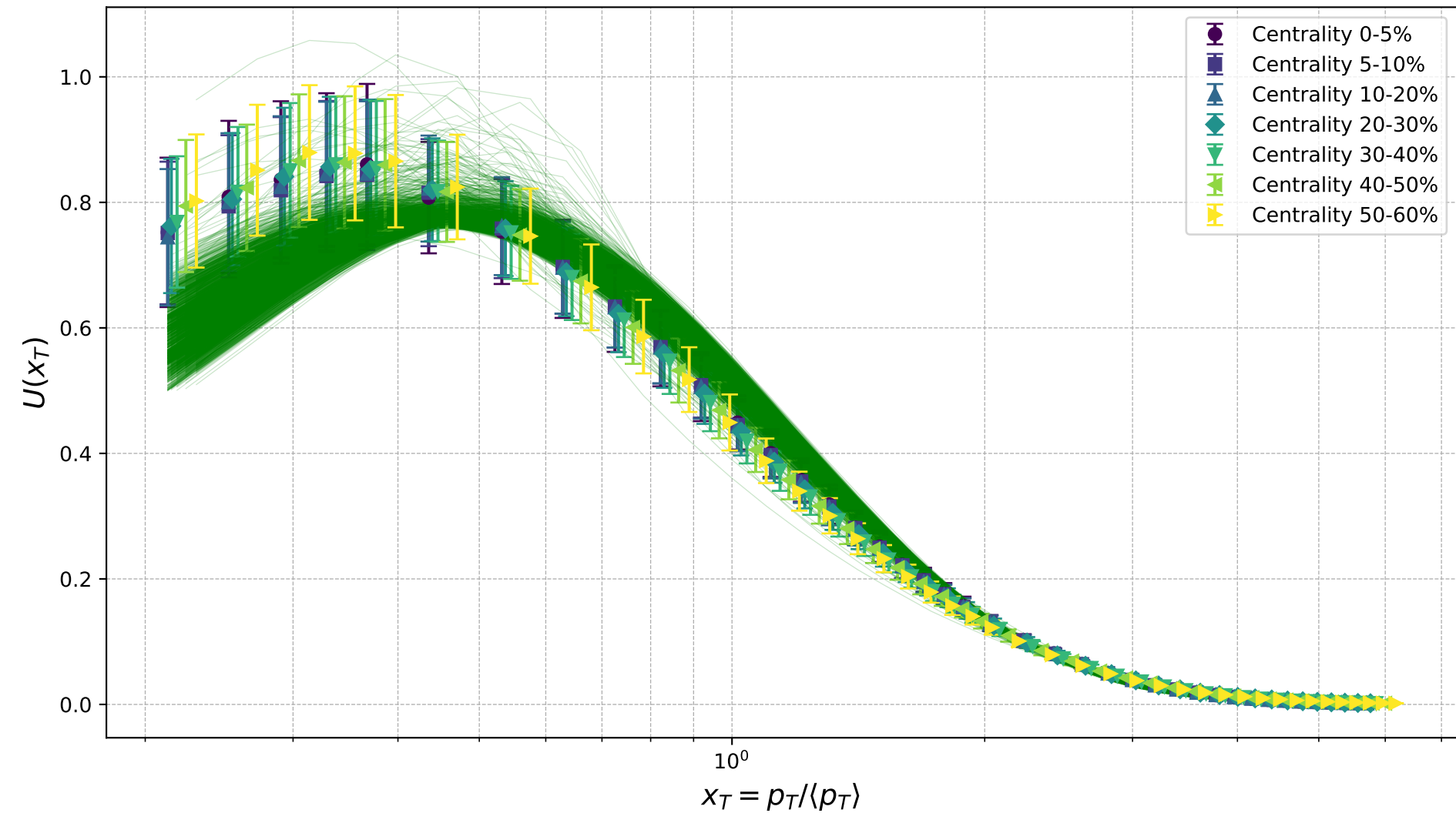
Scaled Spectra U(x_T) for Filtered Design Points PTB Pb-Pb 2.76 TeV
