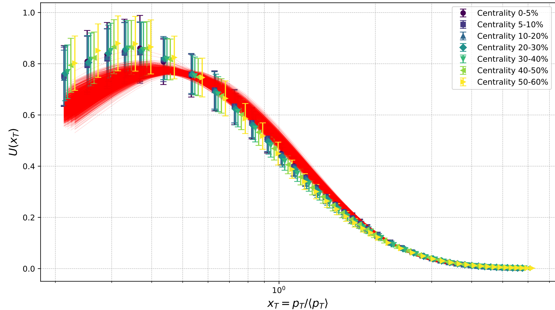
Scaled Spectra U(x_T) for Filtered Design Points CE Pb-Pb 2.76 TeV
