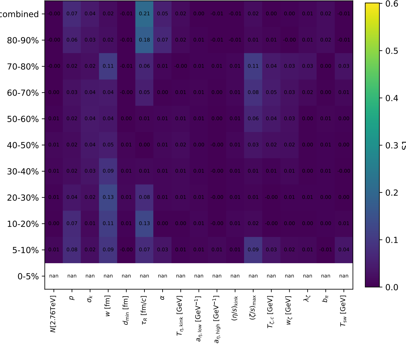
Sobol first-order (S1)
