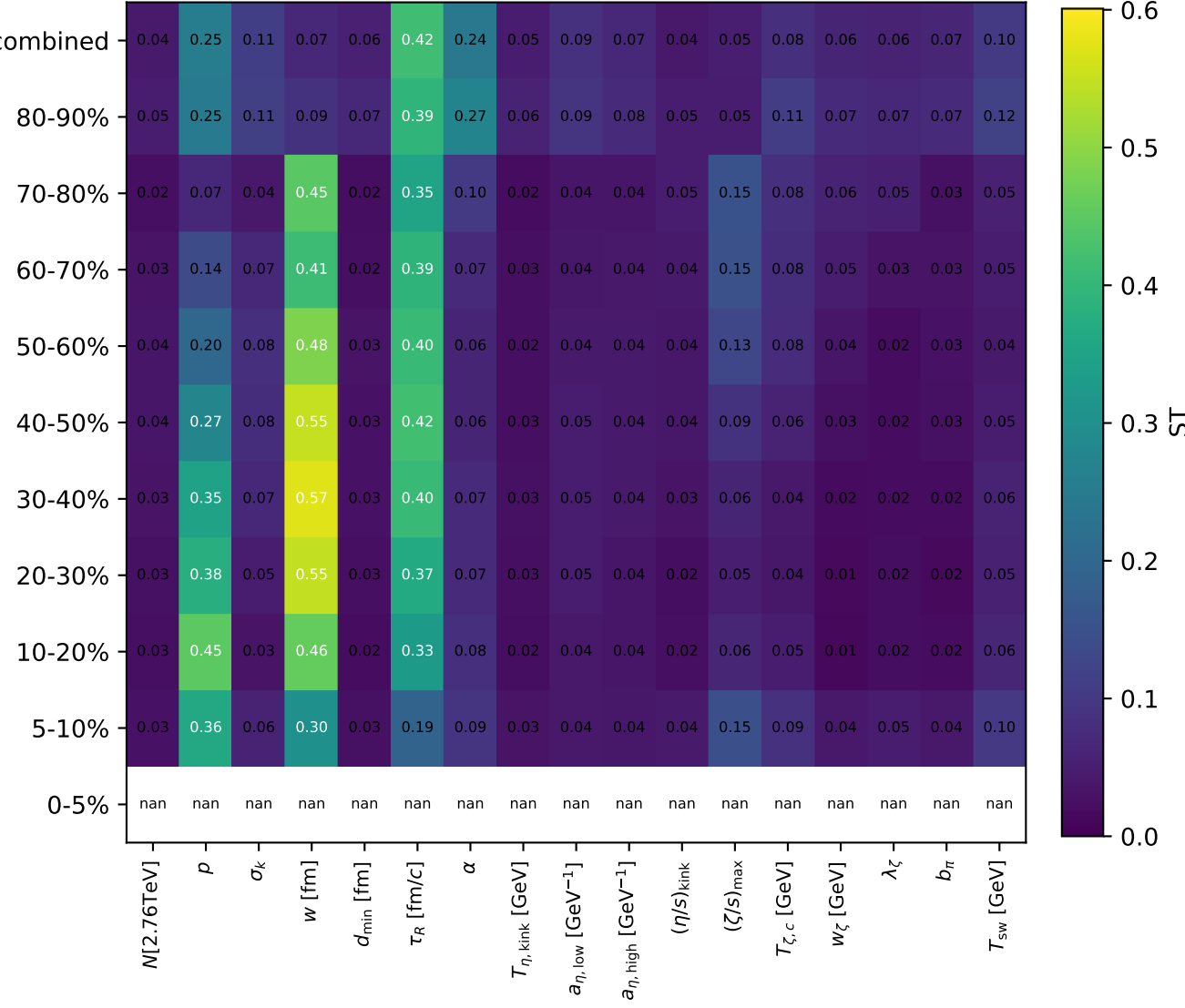
Sobol total-order (ST)
