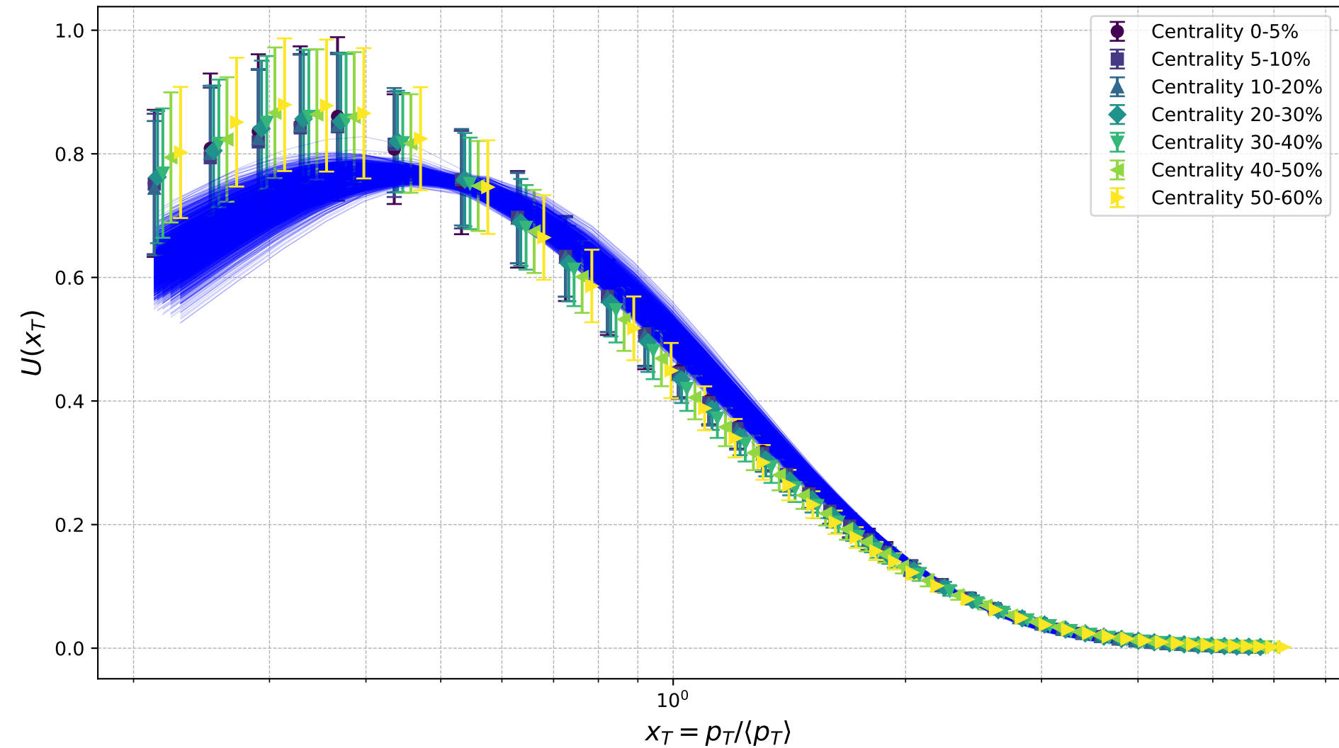
Scaled Spectra U(x_T) for Filtered Design Points Grad Pb-Pb 2.76 TeV
