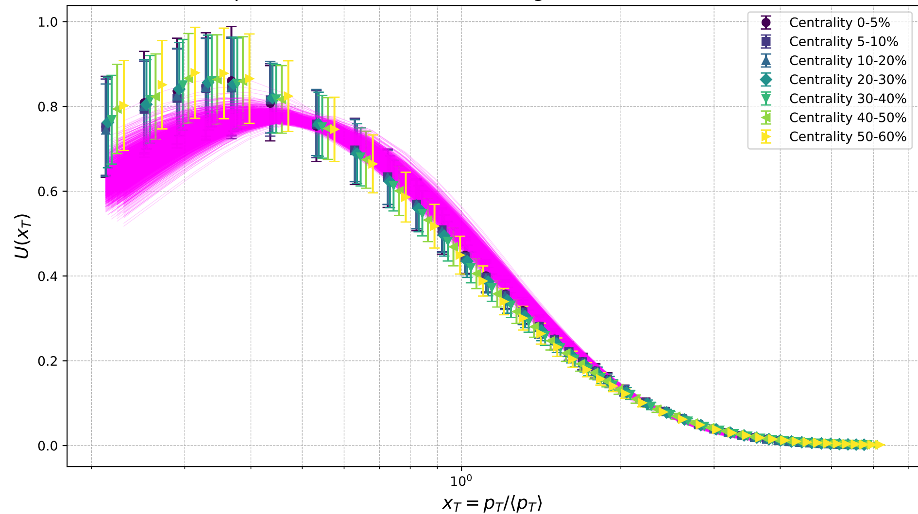
Scaled Spectra U(x_T) for Filtered Design Points PTM Pb-Pb 2.76 TeV
