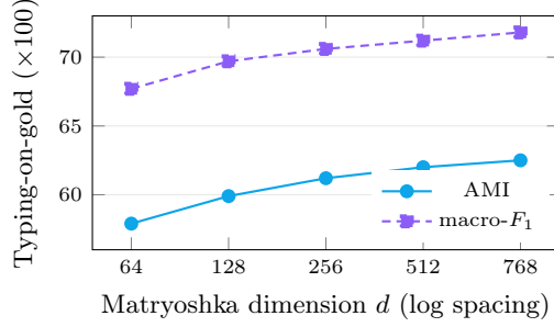
Fig. 6 Typing-on-gold quality vs the Matryoshka truncation dimension d . Both AMI and macro- F_1 degrade smoothly, with diminishing returns rather than a cliff, and flatten above d=256 . Truncation is therefore a graceful cost/quality knob, and the Matryoshka structure survives the contrastive fine-tuning. Data from Table 9 (dimension axis, released seed, 13-set means, log-spaced d )
