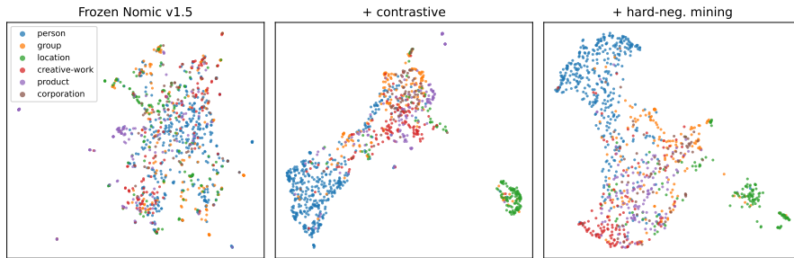
Fig. 2 UMAP of WNUT-17 (held-out) entity embeddings, coloured by gold type, across the three embedder stages: frozen Nomic v1.5, + contrastive fine-tuning, + hard-negative mining. The contrastive stages progressively separate the types into compact clusters on a domain unseen during training
