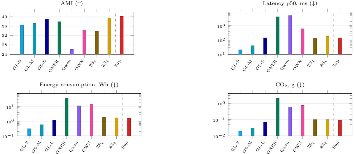
Fig. 6 Per-model means on the four axes (13-set averages, Table 8). The light dotted line separates the zero-shot systems (left) from the supervised OPENER-Sup (right). Latency, energy and CO 2 use a log scale. Labels: GL-S/M/L = GLiNER sizes, OWN = OWNER, ZS i = OPENER-ZS ind , ZS t = OPENER-ZS trans , Sup = OPENER-Sup
