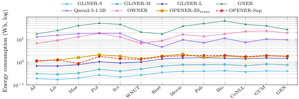
Fig. 5 Per-run energy consumption (Wh, log scale) per dataset (Table 7). Same systems and styling as Figure 3. The OPENER variants sit an order of magnitude below OWNER and the generative GNER/Qwen baselines
