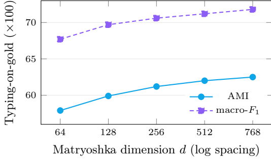
Fig. 7 Typing-on-gold quality vs the Matryoshka truncation dimension d . Both AMI and macro- F_1 degrade smoothly, with diminishing returns rather than a cliff, and flatten above d=256 . Truncation is therefore a graceful cost/quality knob, and the Matryoshka structure survives the contrastive fine-tuning. Data from Table 9 (dimension axis, released seed, 13-set means, log-spaced d )
