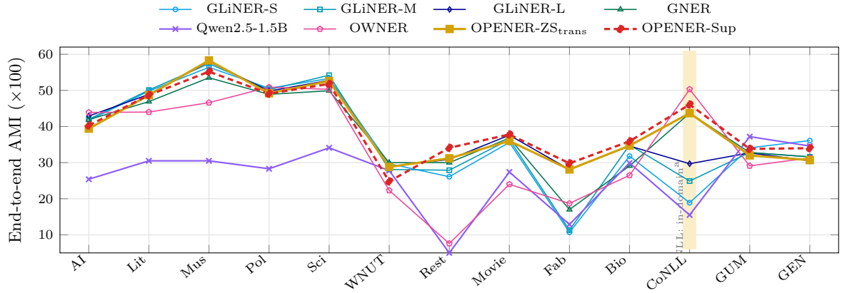
Fig. 3 End-to-end AMI per dataset (Table 5, OPENER curves show the three-seed means). Zero-shot systems are drawn solid. OPENER-Sup is the dashed red line. a CoNLL-2003 (shaded) is in-domain for OWNER and OPENER. b Qwen is evaluated on a 150-sentence subsample per set
