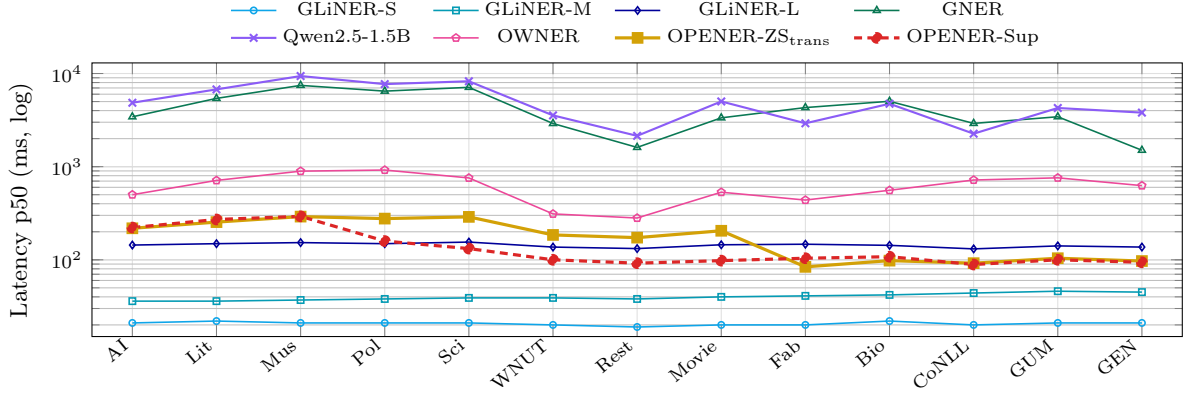
Fig. 4 Per-sentence inference latency (p50, ms, log scale) per dataset (Table 6). Same systems and styling as Figure 3. OPENER-Sup is the dashed red line. The OPENER variants track GLiNER-L, while GNER and the Qwen LLM are one to two orders of magnitude slower
