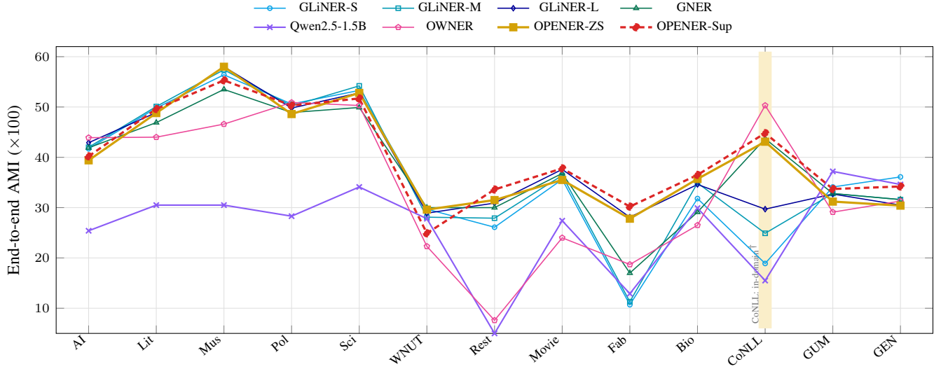
Fig. 2. End-to-end AMI per dataset (Table IV). Zero-shot systems are drawn solid; OPENER-Sup (the supervised upper bound) is the dashed red line. † CoNLL-2003 (shaded) is in-domain for OWNER and OPENER; ‡ Qwen is evaluated on a 150-sentence subsample per set.
