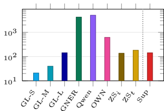
Latency p50, ms ( \downarrow )
